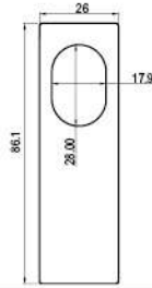
CSD-M18-L M18-L 安装架 Mounting bracket
