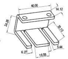
CSD-F40 40x40 安装架 Mounting bracket
